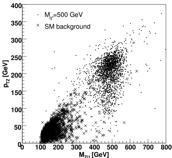
FIG. 3: p_{TZ} vs M_{Zj1} distributions for a resonance of mass of 500 GeV ( \xi = 1 ) and for the SM background. Both the signal and background events passed through complete reconstruction. Each distribution is arbitrarily normalized.
