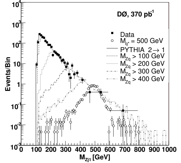
FIG. 2: Invariant mass distribution of the Z boson and the leading jet, M_{Zj1} . The data are shown by the full squares with error bars. The actual number of events in a bin is the product of the plotted value and the bin width measured in 10 GeV units. The SM backgrounds generated with PYTHIA are shown in the histograms: 2 \rightarrow 1 without threshold (solid line), 2 \rightarrow 2 with various M_{Zq} thresholds (discontinuous lines, as indicated). Each curve with a definite M_{Zq} threshold value stops when the curve of the next threshold value takes over. Also shown with open circles is the signal due to an excited quark of 500 GeV mass and narrow width ( \xi = 1 ). The resonance production cross section is taken from Ref. [1].
