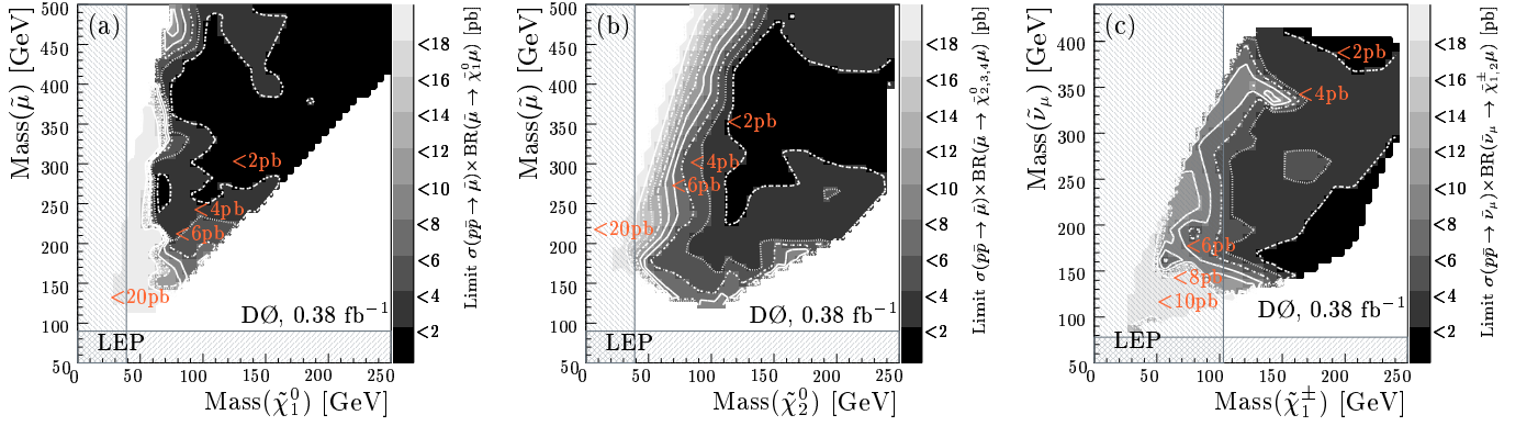
FIG. 2: 95% C.L. limit on slepton production cross section times branching fraction to gaugino plus muon for the channels (i) \tilde{\mu} \rightarrow \tilde{\chi}_1^0 \mu (a), (ii) \tilde{\mu} \rightarrow \tilde{\chi}_{2,3,4}^0 \mu (b) and (iii) \tilde{\nu}_\mu \rightarrow \tilde{\chi}_{1,2}^\pm \mu (c) as a function of slepton and gaugino masses. The darkest region corresponds to a cross section of less than 2 pb. Successively lighter regions have successively higher limits.
