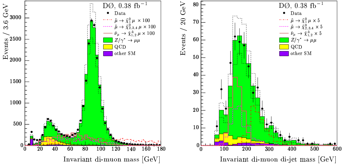
FIG. 1: Invariant di-muon mass in the two-muon sample (a) and reconstructed 4-body mass of two muons and two jets (b). The cascade decays in channels (ii) and (iii) lead to less energy per particle, thus lower invariant masses. The signal expectation for the point with m_{\tilde{t}} = 260 GeV and m_{\tilde{\chi}_1^0} = 100 GeV is scaled in plot (a) by a factor of 100 and in plot (b) by a factor of 5. The dominant SM background is Z/\gamma^* \rightarrow \mu\mu ; other SM backgrounds are Z/\gamma^* \rightarrow \tau\tau ; WW , WZ , ZZ , t\bar{t} and \Upsilon production. The total SM uncertainty is shown as a dashed black line. The data is in good agreement with the SM expectation.
