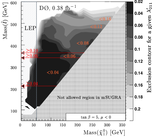
FIG. 3: 95% C.L. exclusion contour on \lambda'_{211} couplings within the mSUGRA framework for \tan \beta = 5 and \mu < 0 . The arrows indicate limits on the slepton mass \tilde{l} , for a given coupling \lambda'_{211} .
