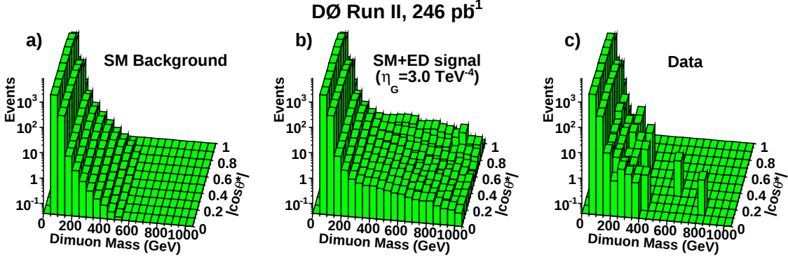
FIG. 2: Two-dimensional distributions in the dimuon mass vs. |\cos \theta^*| for: a) SM background, b) the sum of the SM and large ED contributions for \eta_G = 3 \text{ TeV}^{-4} , and c) data.
