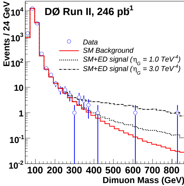
FIG. 3: Comparison between data and SM background in the dimuon mass M , where the effects of ED are enhanced and shown for \eta_G = 1 \text{ TeV}^{-4} and 3 \text{ TeV}^{-4} (dashed lines).
