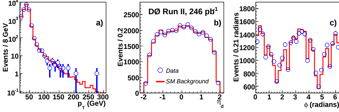
FIG. 1: Comparison of data (circles with error bars) and SM predictions (histogram) in p_T , \eta_d , and \phi [12] of the muons in the event. The dips in the azimuthal angle reflect detector acceptance.
