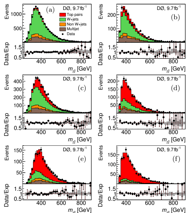
FIG. 4: (Color online). Reconstructed invariant mass of the top quark-antiquark pair, m_{t\bar{t}} . The left column shows l+\geq 3 jet events, and the right column shows l+\geq 4 jet events. Rows from top to bottom display events with 0, 1, and \geq 2 b tags. The ratio between the data counts and the model expectation is shown in the lower panels, with the hashed area representing the systematic uncertainties.
