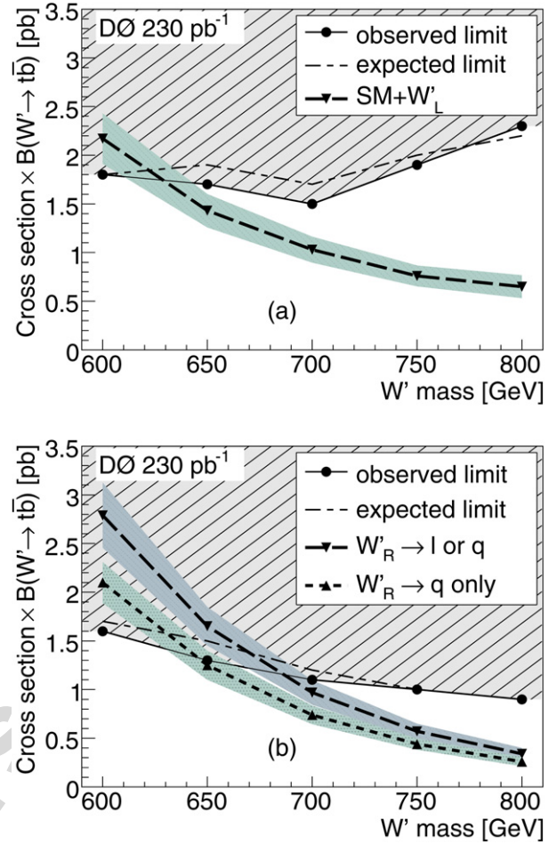
Fig. 4. Cross section limits at the 95% confidence level versus the mass of the W' boson with (a) left-handed couplings and (b) right-handed couplings. Also shown are the NLO cross sections according to Table 1 and the expected limits. The shaded regions above the circles are excluded by this measurement.
