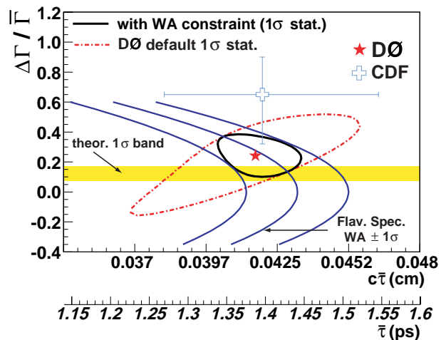
FIG. 4: The DØ default one- \sigma (stat.) contour ( \delta \ln(L) = 0.5 ) compared to a one- \sigma band for the world average (WA) measurement based on flavor-specific decays, \tau_{fs} = 1.442 \pm 0.066 ps. A simultaneous fit to our data and the WA gives a one- \sigma range \bar{\tau}(B_s^0) = 1.39 \pm 0.06 ps and \Delta\Gamma/\bar{\Gamma} = 0.25^{+0.14}_{-0.15} . The SM theoretical prediction is shown as the horizontal band.
